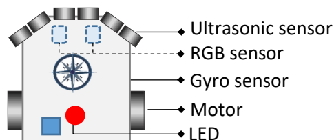
Figure 9: ROBOT configuration
